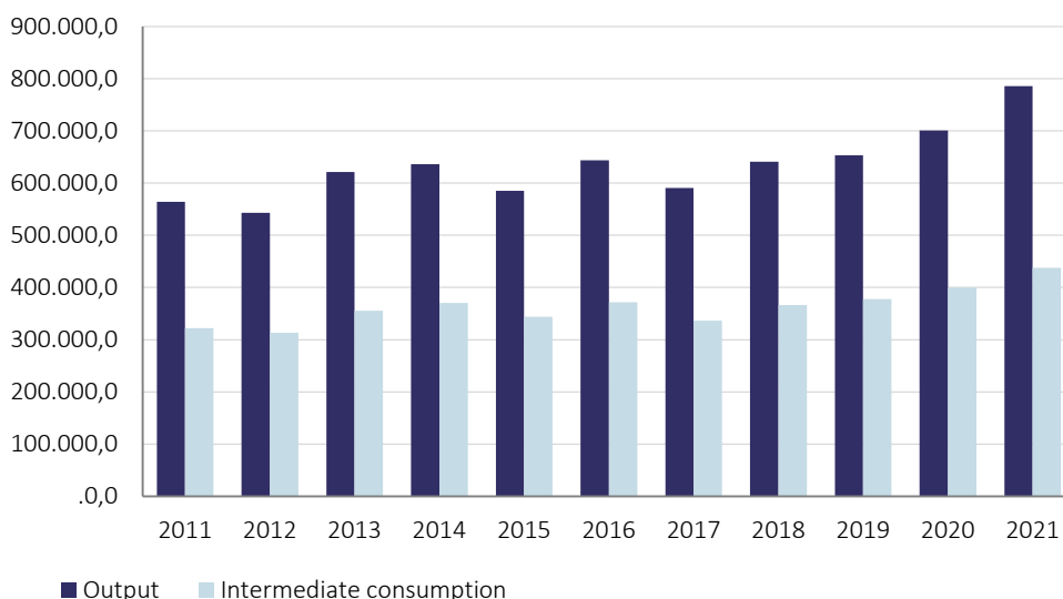
Graph 4.2. Output and intermediate consumption at current prices, 2011 – 2021, RSD million
