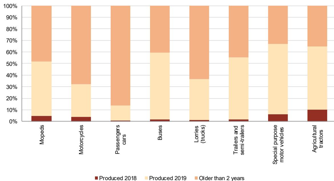
Age structure of first time registered road motor vehicles - Republic of Serbia -
