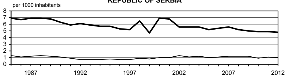
Mariages and divorces in the period 1985-2012 REPUBLIC OF SERBIA
