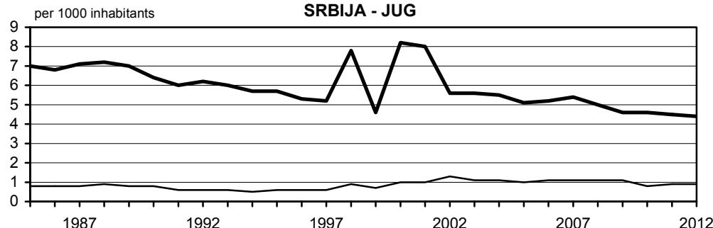
Mariages and divorces in the period 1985-2012 SRBIJA - JUG
