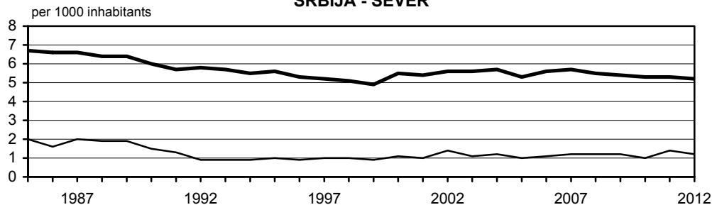
Mariages and divorces in the period 1985-2012 SRBIJA - SEVER
